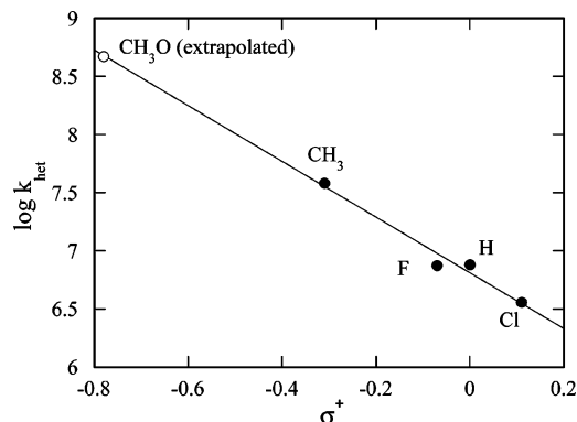
FIGURE 5. Correlation analysis of rate constant k_{het} in acidic HFIP as a function of \sigma^+ 51 for the elimination of water from \beta -OH radicals 2a–d . The data point for radical 2e was estimated by using the slope and \sigma^+(\text{CH}_3\text{O}) = -0.78 .
